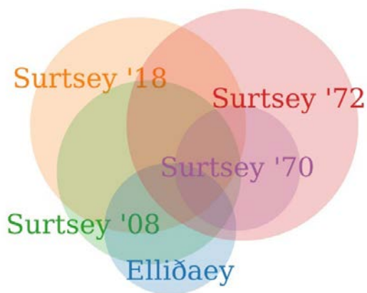
Figure 7. Area proportional Venn diagram for the total number of taxa (Appendix B) found on Surtsey in the surveys in 1970, 1972, 2008 and 2018. Each circle represents a total species number for a given year: 1970 = 17, 1972 = 72, 2008 = 39, 2018 = 59; the intersections indicate the species in common.
