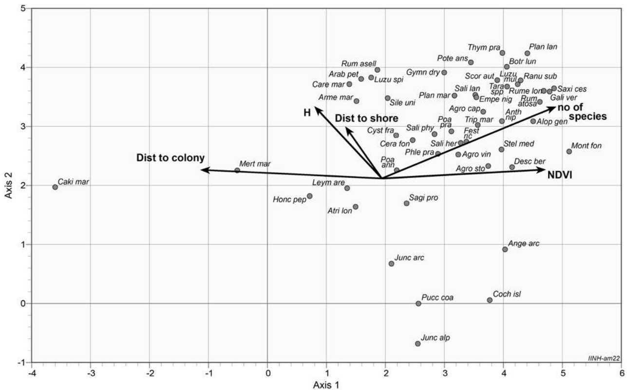
Fig. 9. Results of DCA-ordination of species based on species abundance in quadrats measured in 1996-1997, 2005-2006 and 2014-2015. Only 50 species with the greatest effect on the ordination are shown. Relationship between environmental variables and the DCA-ordination is denoted with arrows where arrow length indicates the relative importance of the variables in explaining the vegetational variation. H is the height (m) above sea level measured in 1998. Full names of the species are given in Appendix I.
